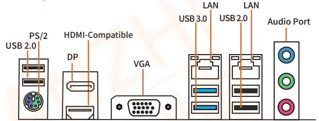
1-2 Overall Rear I/O Panel Display
