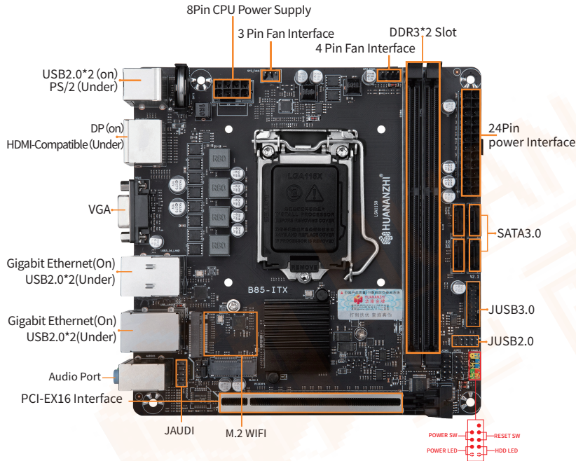
1-1 B85-ITX MotherBoard Illustration
